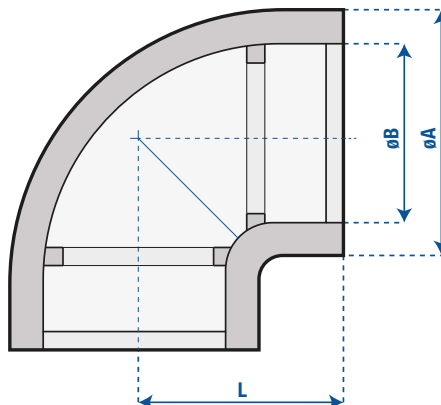
Elbow 90 Equal Banded Socket Weld
