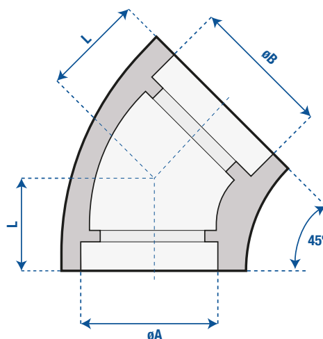
Elbow 45 Banded Socket Weld
