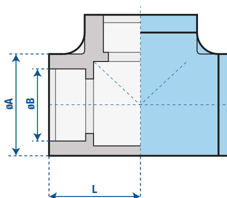
Tee Banded Socket Weld
